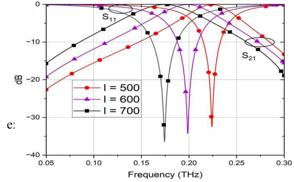
Fig. 4: Parametric analysis of the bandpass filter with vary-ing cross lengths: Transmission (S21) and reflection (S11) responses
