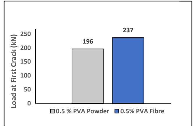
Fig. 11. Average Crack Initiation Load Comparison of Retrofitted Columns
