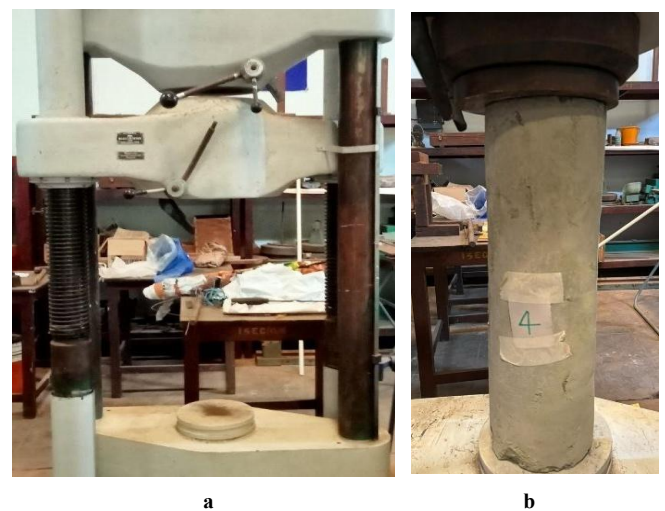
Fig. 9 (a) Universal Testing Machine (b) Test Setup of Sample Column
